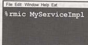
MyServiceImpl_Stub.class
